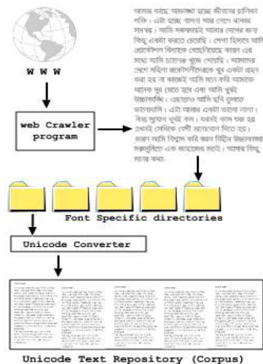
Figure 1: The automatic Bangla corpus creation process.
